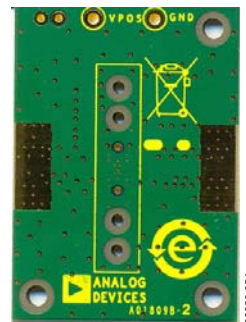
Figure 55. Evaluation Board Layout (Bottom View)
