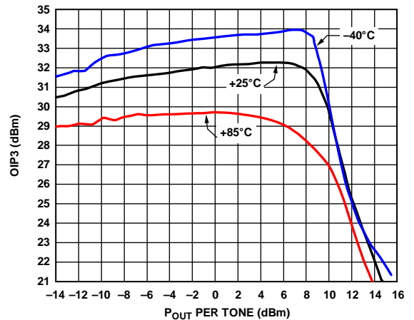
Figure 50. OIP3 vs. Output Power (P OUT ) and Temperature
