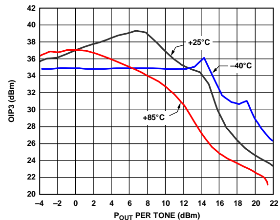
Figure 8. OIP3 vs. Output Power ( P_{out} ) and Temperature
