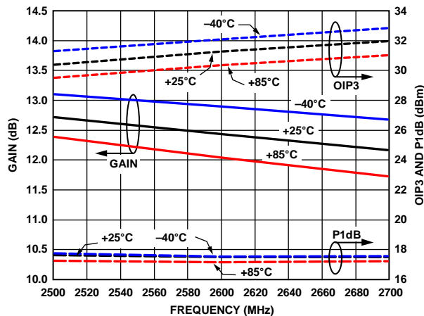
Figure 43. Gain, OIP3, and P1dB vs. Temperature
