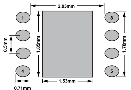
Figure 56. Recommended Land Pattern
